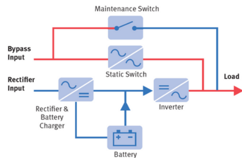
Dual Input System Principal Diagram
