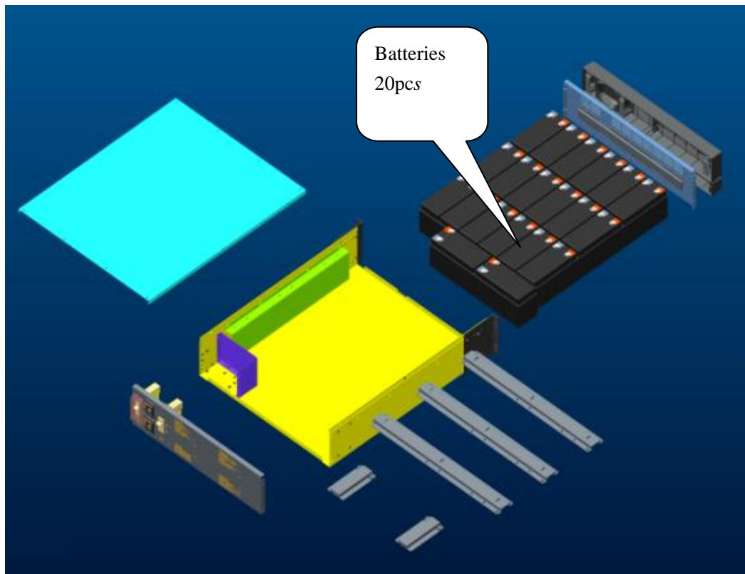
Fig. 4 (20pcs batteries installation)
